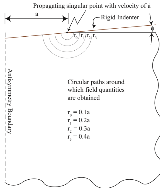
Fig. 5. Circular paths along which field quantities are reported, where a is the distance of the contact point singularity from the antisymmetry boundary, and \dot{a} is the rate of motion of contact point singularity with respect to time. Radii of paths are r_0 = 0.1a , r_1 = 0.2a , r_2 = 0.3a , and r_3 = 0.4a .
