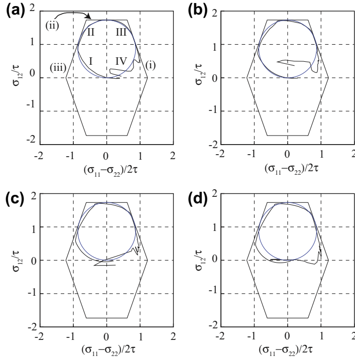
Fig. 9. Stress trajectories in vicinity of contact point singularity for various radii: (a) r_0 = 0.1a ; (b) r_1 = 0.2a ; (c) r_2 = 0.3a ; and, (d) r_3 = 0.4a . Blue lines indicate analytical predictions and black lines indicate numerical results.
