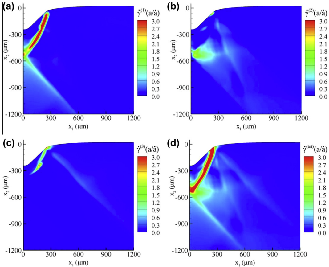
Fig. 17. Increment of plastic slip, \dot{\gamma}^{(i)} a / \dot{a} , on effective in-plane slip systems: (a) Slip System (i); (b) Slip System (ii); (c) Slip System (iii); (d) Total from all slip systems.
