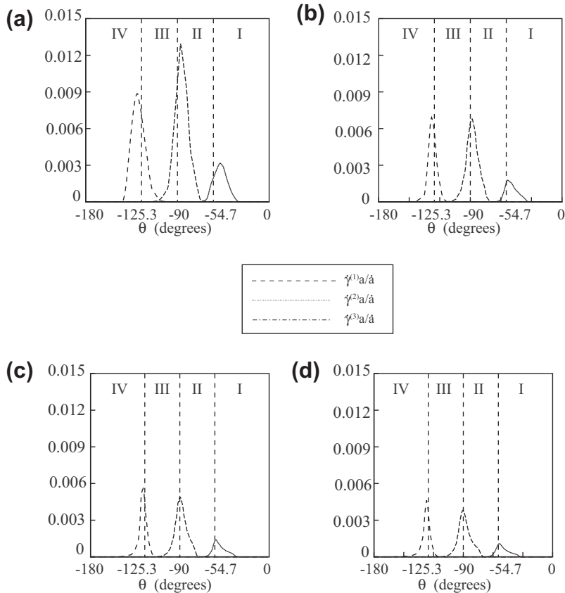
Fig. 11. Slip increments as a function of angle and radius with respect to the contact point singularity: (a) r_0 = 0.1a ; (b) r_1 = 0.2a ; (c) r_2 = 0.3a ; and, (d) r_3 = 0.4a .
