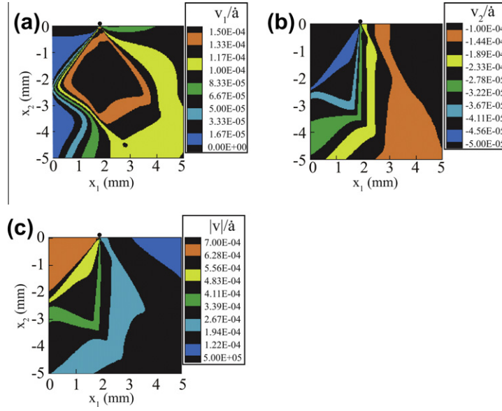
Fig. 12. Normalized velocity fields: (a) v_1/\dot{a} ; (b) v_2/\dot{a} ; and, (c) |v|/\dot{a} .
