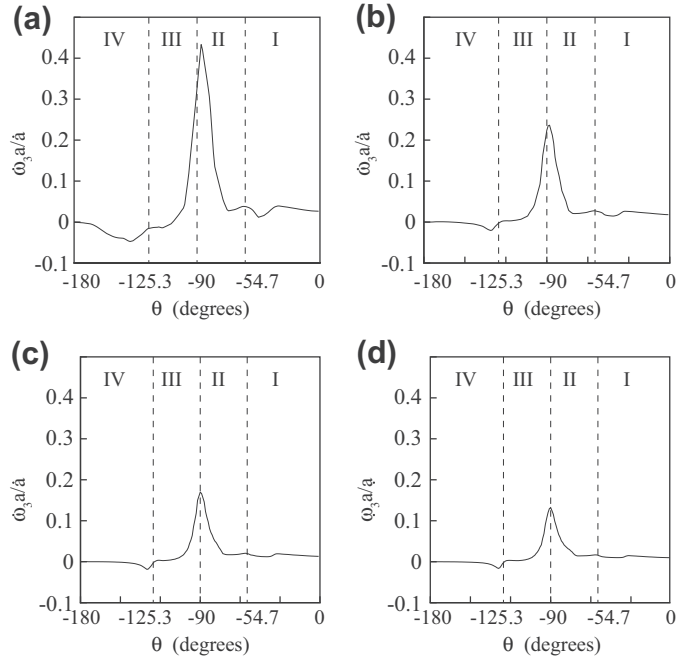
Fig. 15. Normalized lattice rotation rates, \dot{\omega}_3 a / \dot{a} , as a function of angle and radius with respect to the contact point singularity: (a) r_0 = 0.1a ; (b) r_1 = 0.2a ; (c) r_2 = 0.3a ; and, (d) r_3 = 0.4a .
