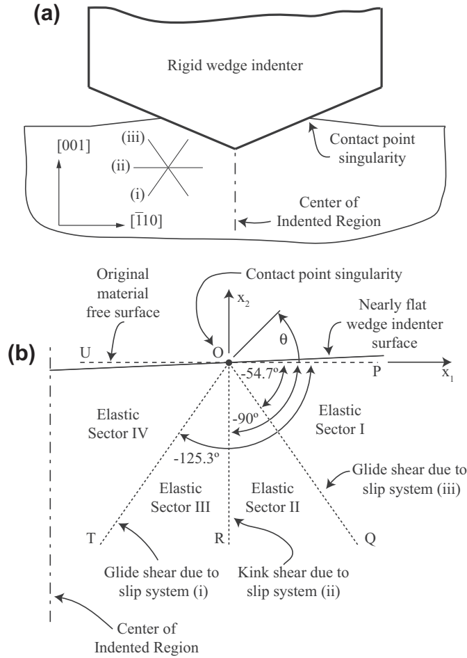
Fig. 2. Wedge indentation into single FCC crystal: (a) orientations of effective slips systems; and, (b) predicted asymptotic deformation field under the contact point singularity.
