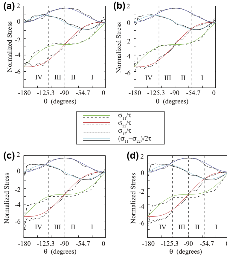
Fig. 8. Stress components as a function of angle and radius with respect to the contact point singularity: (a) r_0 = 0.1a ; (b) r_1 = 0.2a ; (c) r_2 = 0.3a ; and, (d) r_3 = 0.4a . Colored lines indicate analytical predictions and black lines indicate numerical results.
