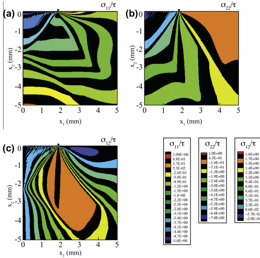
Fig. 7. Contours of stress components associated with quasistatically propagating contact point singularity: (a) \sigma_{11}/\tau ; (b) \sigma_{22}/\tau ; and, (c) \sigma_{12}/\tau . The instantaneous position of the contact point singularity is indicated by a small circle in each plot.
