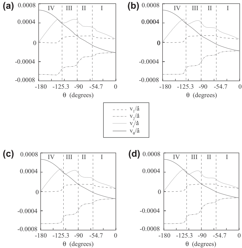
Fig. 13. Normalized velocities as a function of angle and radius with respect to the contact point singularity: (a) r_0 = 0.1a ; (b) r_1 = 0.2a ; (c) r_2 = 0.3a ; and, (d) r_3 = 0.4a .
