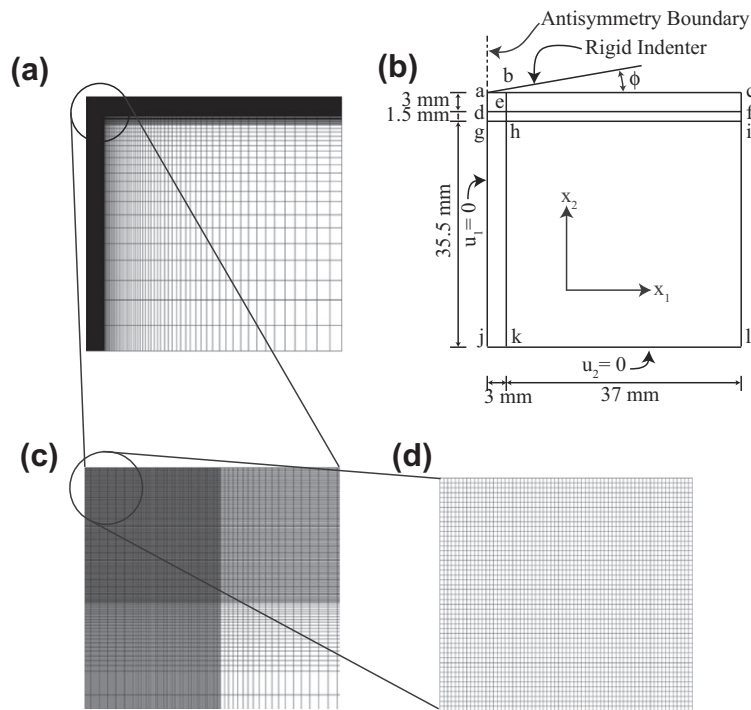
Fig. 4. Mesh detail of finite element simulation: (a) overall mesh; (b) schematic representation showing various regions of mesh along with the indenter surface; (c) close-up view of mesh; and, (d) region of mesh penetrated by indenter surface.
