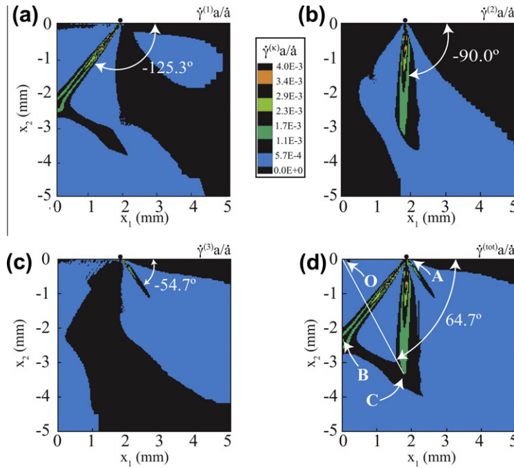
Fig. 10. Normalized slip increments \dot{\gamma}^{(\kappa)}a/\dot{a} on: (a) slip system (i); (b) slip system (ii); (c) slip system (iii); (d) sum of slip increments on three effective in-plane slip systems, where characteristic points of the slip increment field are indicated.
