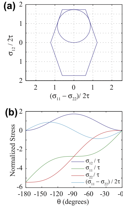
Fig. 3. Asymptotic stress field around contact point singularity for nearly-flat wedge in FCC single crystal: (a) trajectory in stress space; and, (b) angular variation of individual stress components.
