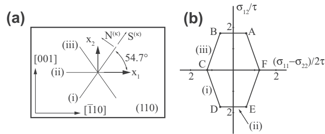
Fig. 1. Effective in-plane plastic slip systems of FCC crystal: (a) orientations of effective slips systems relative to external surface of indented crystal; and, (b) plastic yield surface associated with in-plane deformation, where the effective in-plane slip system associated with each pair of parallel sides of the yield surface is indicated.
