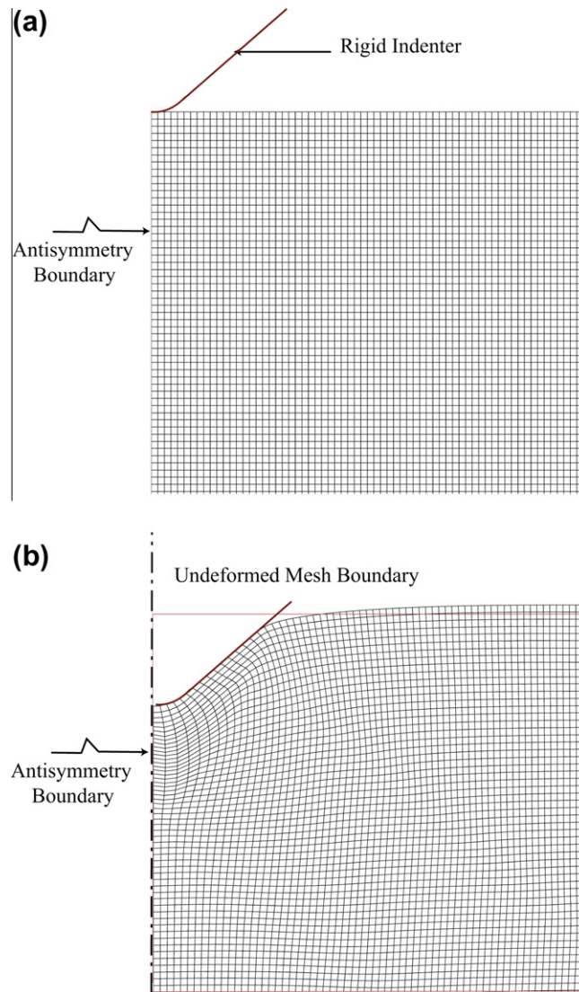
Fig. 16. Finite element mesh for wedge indentation with 90° included angle: (a) Geometry of mesh and rigid indenter; (b) Deformed mesh after indentation to depth of 250 μm.
