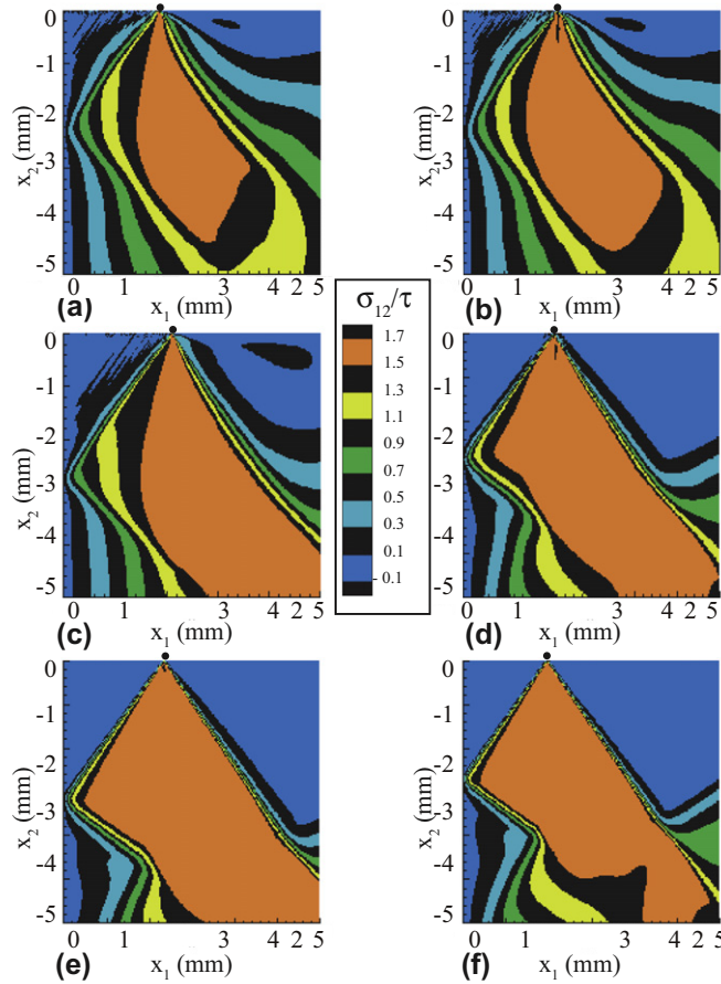
Fig. 6. The \sigma_{12} stress field transition for different \phi : (a) \phi = 0.0191^\circ ; (b) \phi = 0.0382^\circ ; (c) \phi = 0.0764^\circ ; (d) \phi = 0.1528^\circ ; (e) \phi = 0.3056^\circ ; and (f) \phi = 0.6112^\circ . The instantaneous position of the contact point singularity is indicated by a small circle in each plot.
