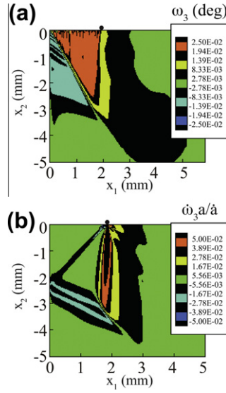
Fig. 14. Rotation of crystal lattice: (a) lattice rotation in degrees; (b) normalized lattice rotation rate, \dot{\omega}_3 a / \dot{a} .
